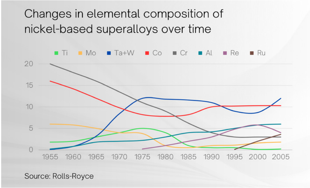
Changes in elemental composition of nickel-based superalloys over time (Source: Rolls-Royce 37 )
