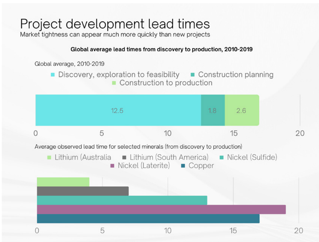
Average observed lead time for selected minerals (from discovery to production). It is a long way to sourcing and self-sufficiency. Research and innovation can help accelerate this development and making mining and metallurgy more competitive in Europe (IAE, 2020).
