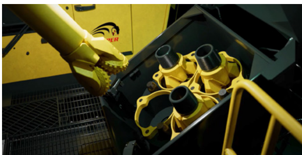
Automatic Bit Changer ABC (Credit: EPIROC)
